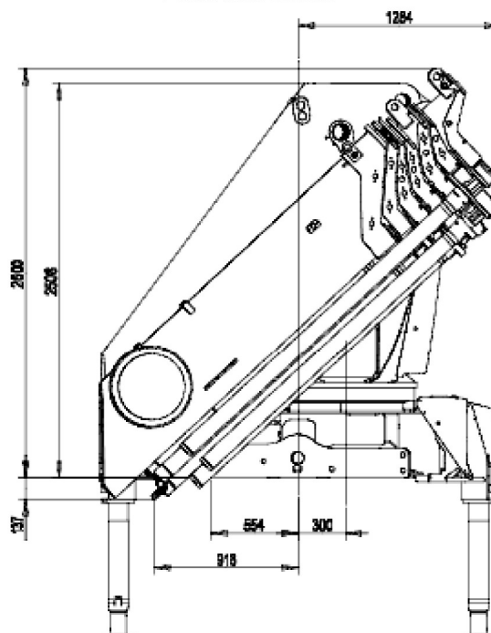
Front view folded
