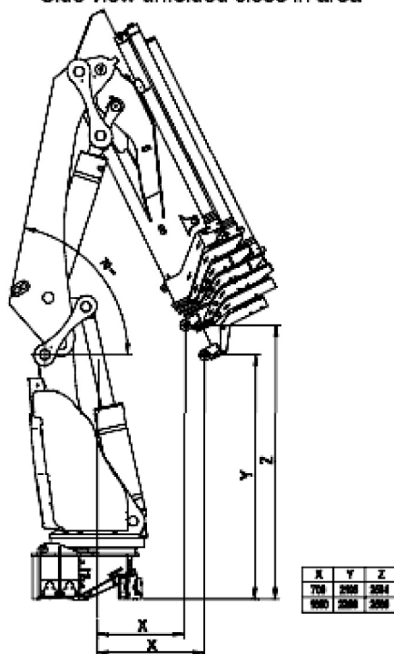
Side view unfolded close in area
