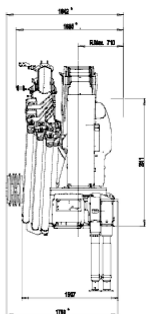
Side view folded
